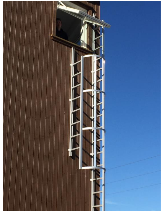
Open MODUM ladder with Back protection
